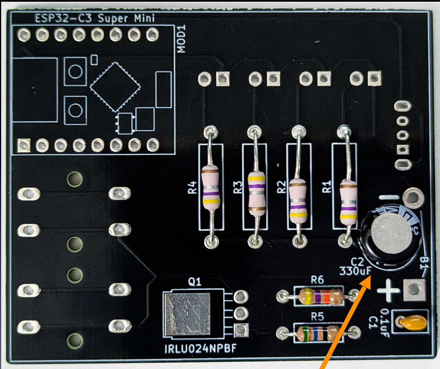
Capacitor C2
